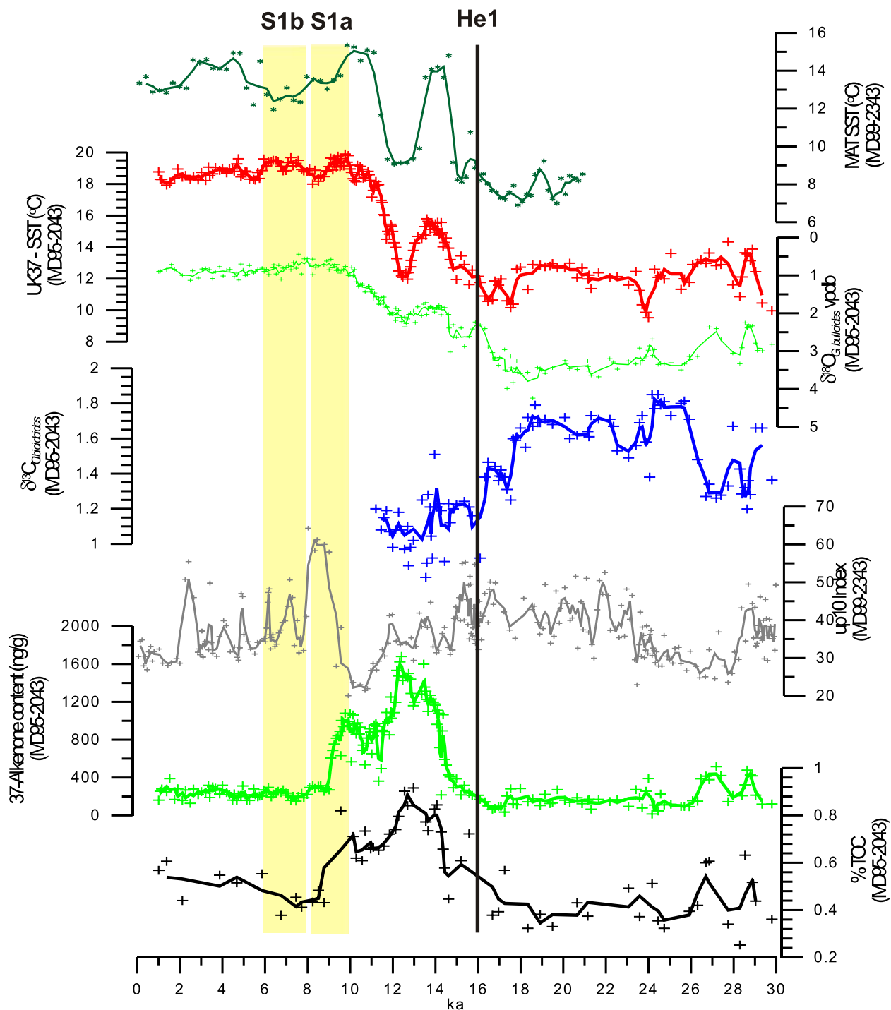
Figure 4. Indicators of bottom ventilation in the Alboran Sea from core MD95-2043 during the last deglaciation. Also shown is the bottom velocity (UP10) record from MD99-2343 [Frigola et al. , 2008] and the winter SST record for the same core. All methods are described in section 3.2. Lines represent 3-point moving averages. The duration of deposition of sapropel 1 is indicated, including the duration of the interruption.
